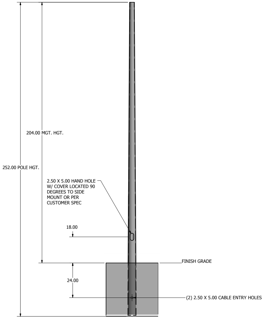
POLE DETAIL
